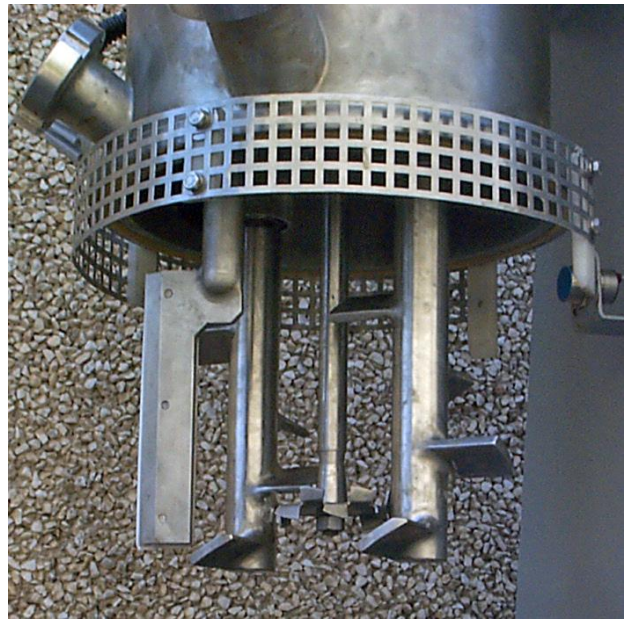
Mixing Tools of Double Planetary Mixer
